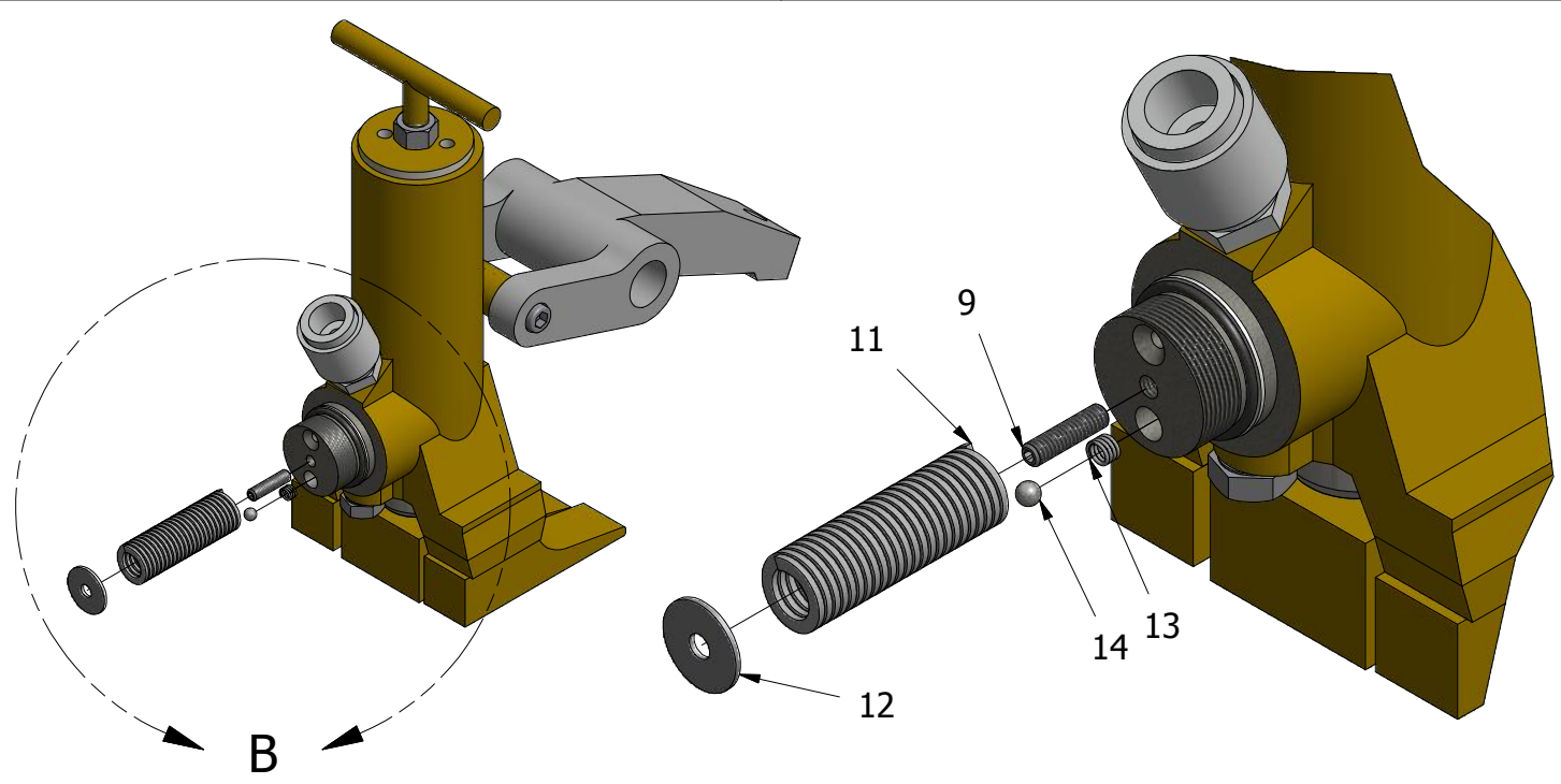
DETAIL B SCALE 1 / 2
